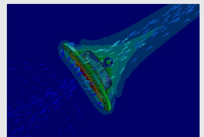
Thermal Air Flow
